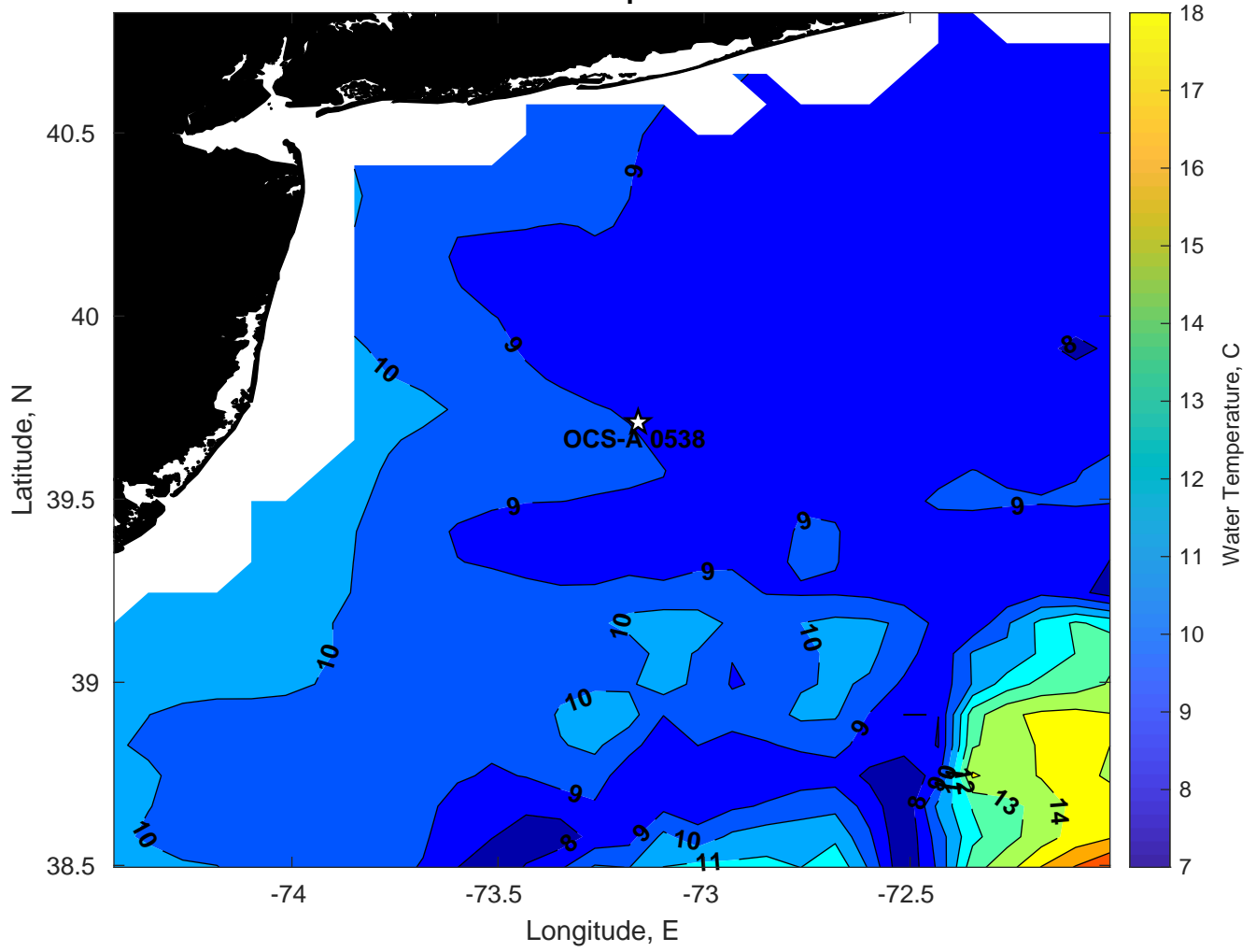
SST for OCS-A 0538 at 18-Apr-2024 00:00:00
